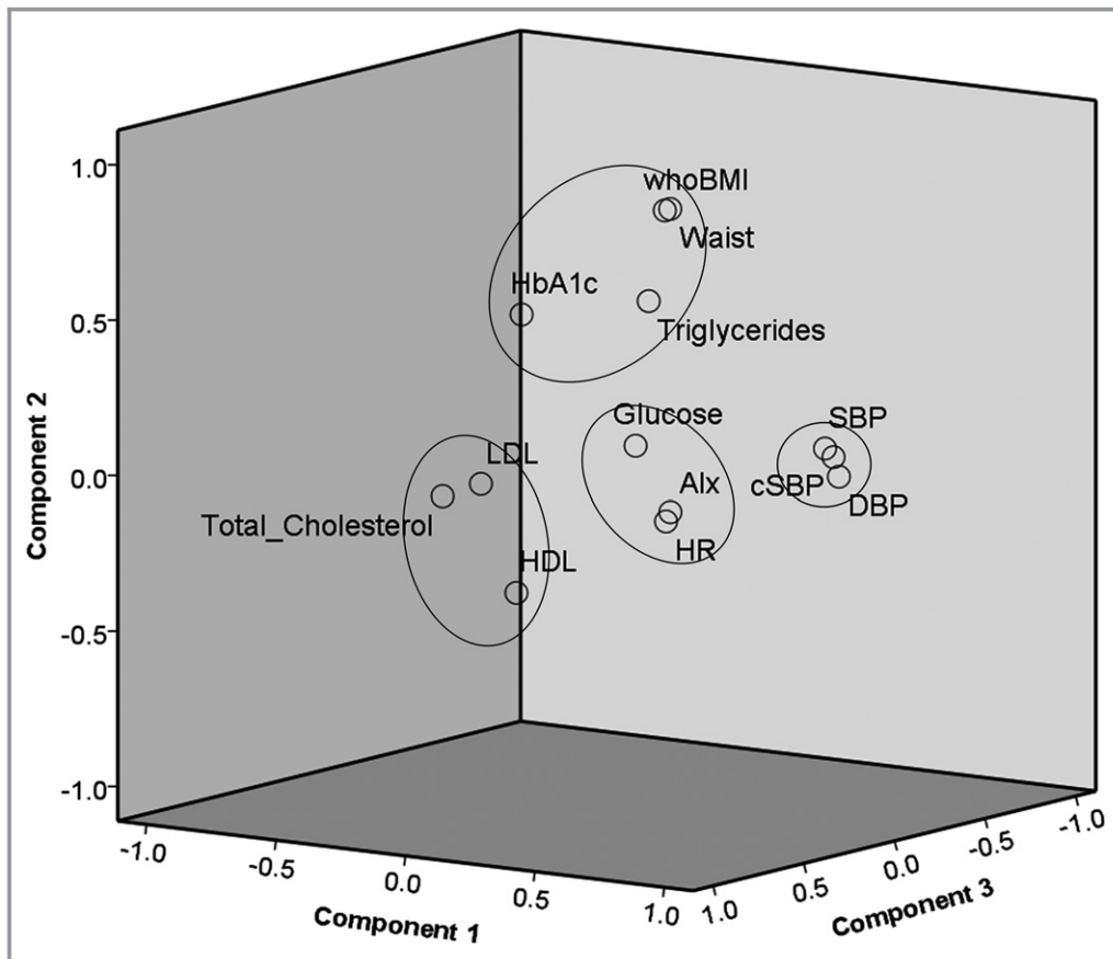
Figure. Component plots with factor diagrams from principle component analysis with varimax rotation. Alx indicates augmentation index; cSBP, central systolic blood pressure; DBP, diastolic blood pressure; HbA1c, glycated hemoglobin; HDL, high-density lipoprotein; HR, heart rate; LDL, low-density lipoprotein; SBP, systolic blood pressure; whoBMI, body mass index z scores, calculated using the 2007 World Health Organization method.
