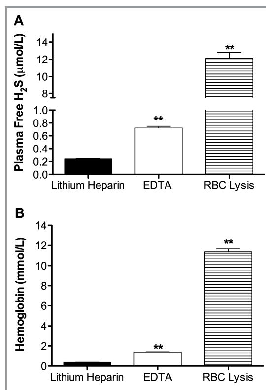
Figure 2. Effect of blood collection tubes on plasma hydrogen sulfide (H 2 S) levels. Venous blood was collected from healthy volunteers in either lithium heparin or ethylenediaminetetraacetic acid (EDTA) vacutainer collection tubes. A, reports the differences in plasma free H 2 S between the different collection tubes vs lysed red blood cells (RBC) (** P <0.01 vs lithium heparin collection tubes). B, illustrates amount of cell free hemoglobin measured using the Drabkin assay in plasma from blood collected in various tubes vs lysed red blood cells (** P <0.01 vs lithium heparin collection tubes).
