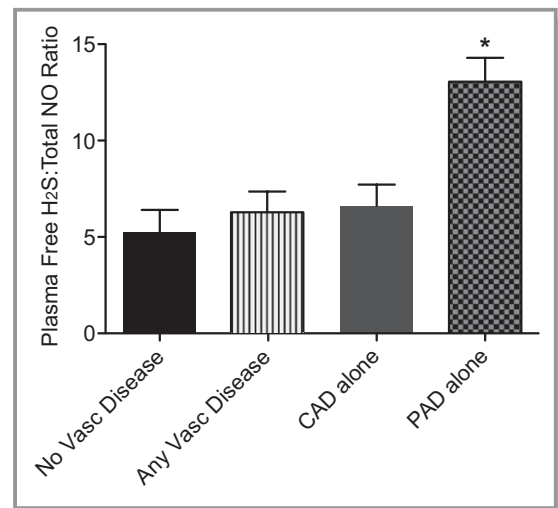
Figure 3. Plasma-free hydrogen sulfide to total NO ratio by vascular disease. The ratio of plasma-free hydrogen sulfide to total NO was calculated per vascular disease cohort. Free H 2 S:NOx ratio was significantly elevated in patients with PAD alone over all other comparison cohorts, * P <0.05. No vascular disease n=53, CAD alone n=66, PAD alone n=13, and any vascular disease n=140. CAD indicates coronary artery disease; H 2 S, hydrogen sulfide; NO, nitric oxide; PAD, peripheral artery disease.
